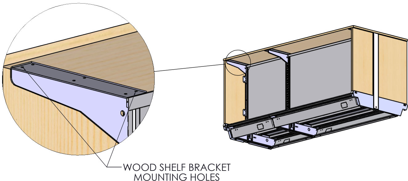
DETAIL C SCALE 1 : 4
